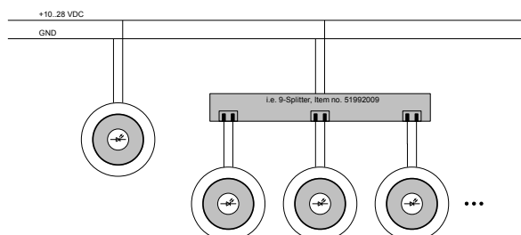
Anschlussskizze Bari CV Connection drawing Bari CV
